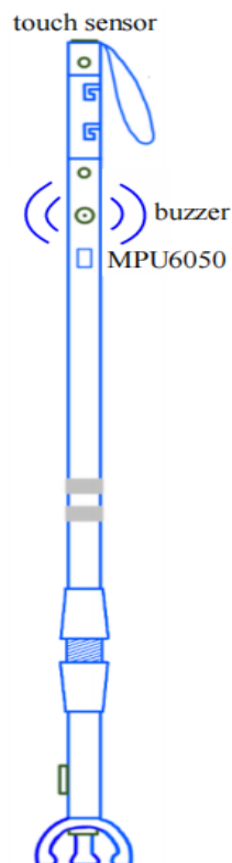
Fig. 5. Fall detection
