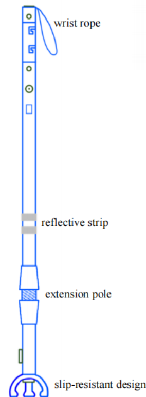
Fig. 6. Extra features
