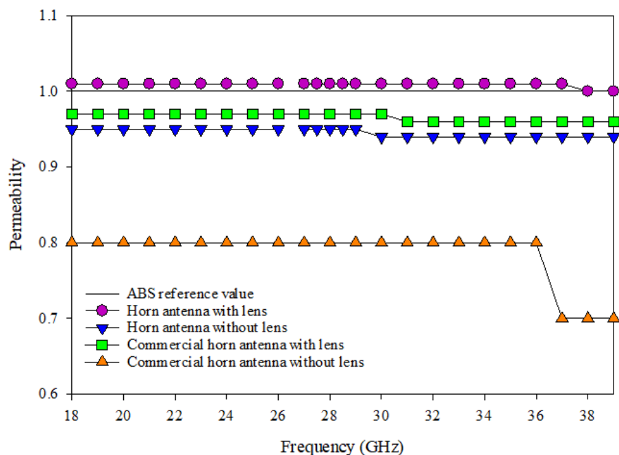
Fig. 22. \mu_r of ABS with and without lens
